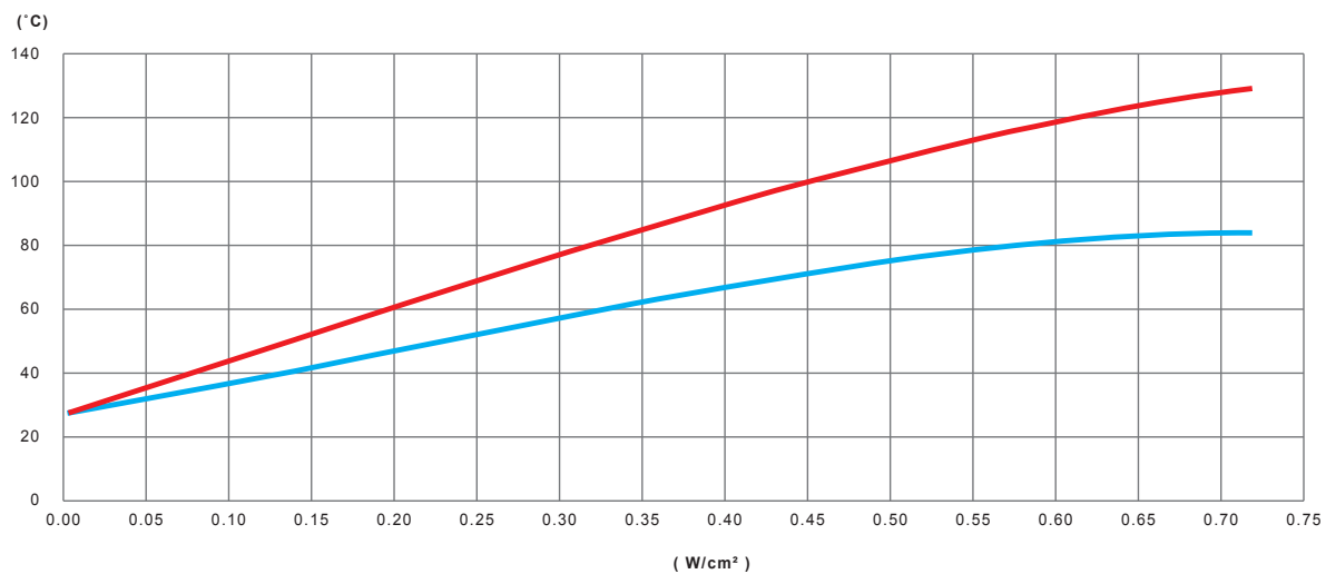
Variation, as a function of the power in W/cm² of the silicone heating ribbon, of the wall temperature of a PVC tube filled with non-circulating water, non-thermally insulated
