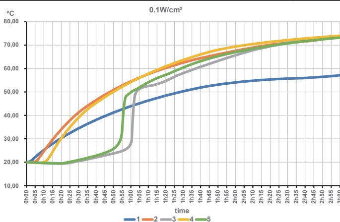
With a surface load of 0.1W/cm 2 (60W)
