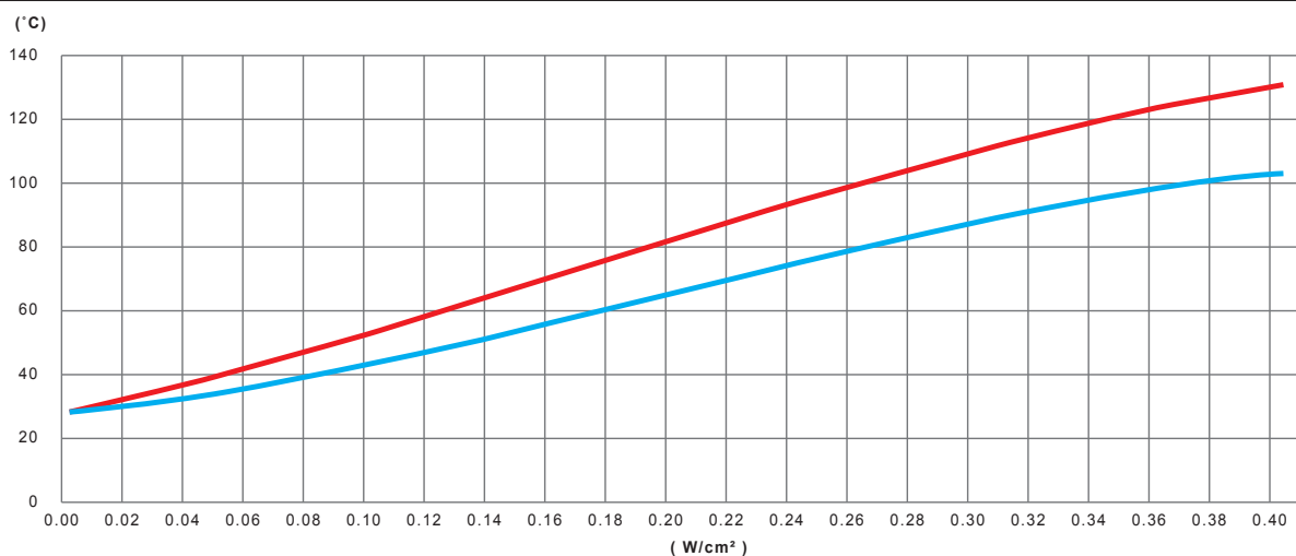
Variation, as a function of the power in W/cm² of the silicone heating ribbon, of the wall temperature of a PVC tube filled with non-circulating water, thermally insulated by 20mm PVC-NBR foam
