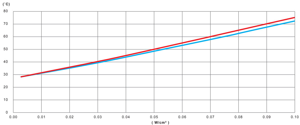
Variation, as a function of the power in W/cm² of the silicone heating ribbon, of the wall temperature of an empty PVC tube, thermally insulated by 20mm of PVC-NBR foam
