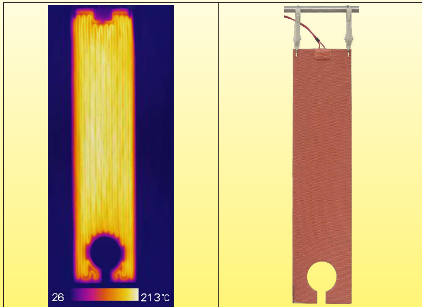
Thermographic image of a 2.4mm flat silicone heater with a 1\text{W}/\text{cm}^2 surface power load, suspended in calm air, not fixed on a board, at an ambient temperature of 25^\circ\text{C} . The surface temperature reaches 213^\circ\text{C} , nearby its destruction.
